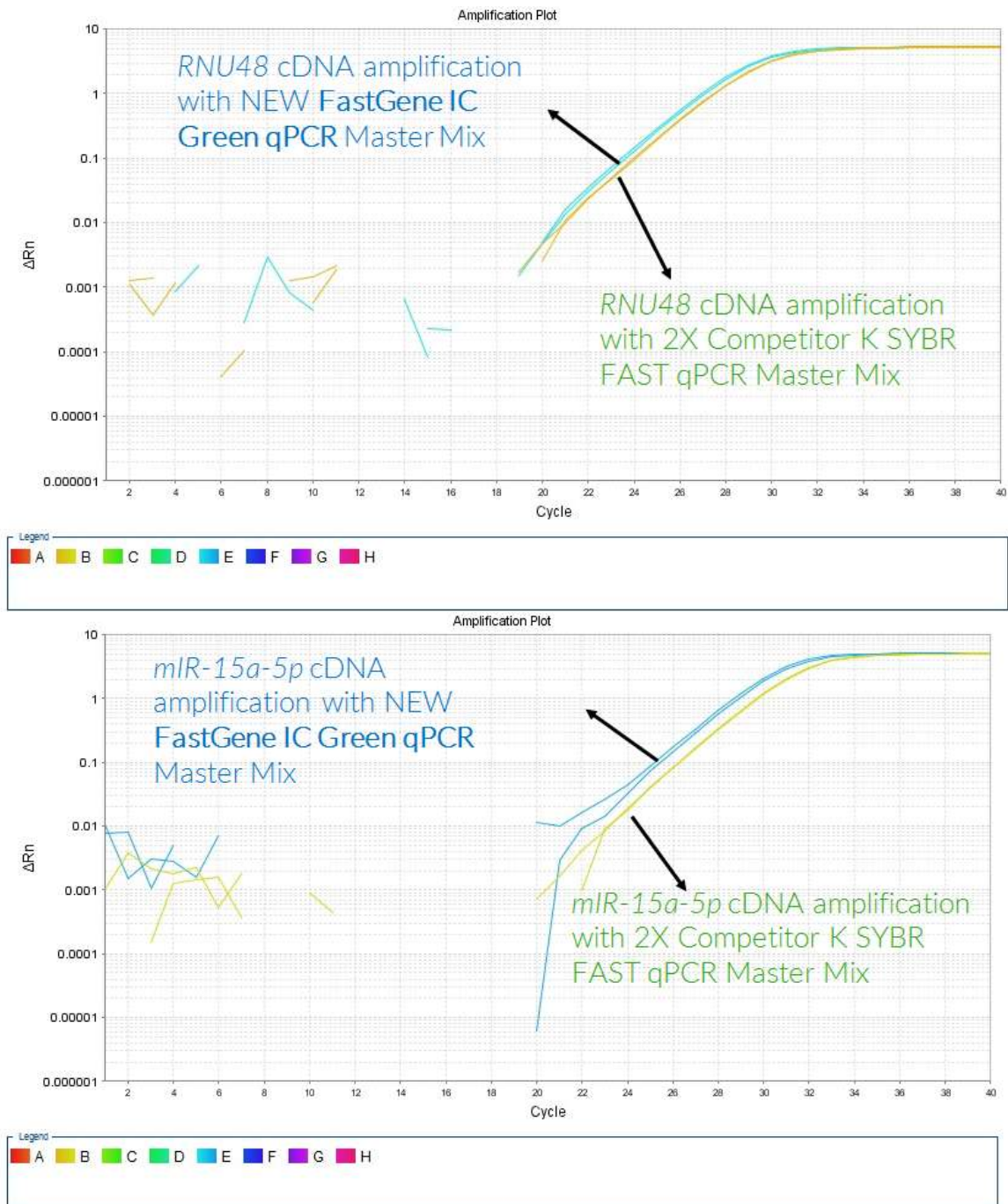
Fig. 2: Comparison of FastGene ® IC Green (blue) with the market leading competitors KB (yellow). The differences of the CT-values were under 1 cycle. Data was kindly provided by an independent researcher.
